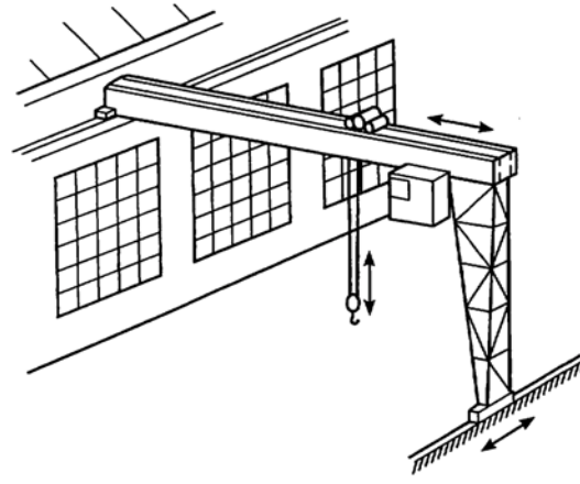
Fig. 4 Semigantry Crane
